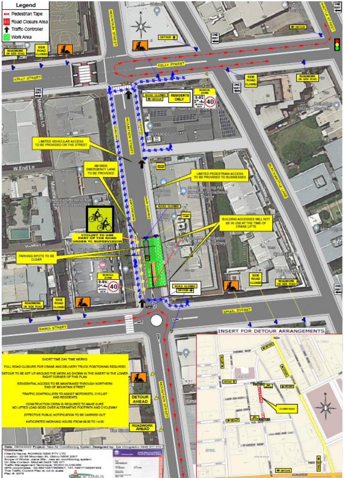
Appendices – Figure 4 – Traffic Guidance Scheme - TGS #3376
